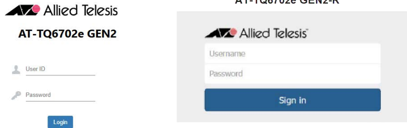
Figure 38. Login Window
