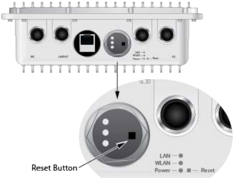
Figure 5. Reset Button
