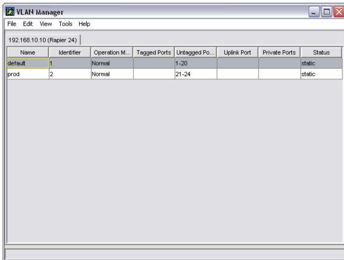
New VLAN definition added to VLAN Information Window
