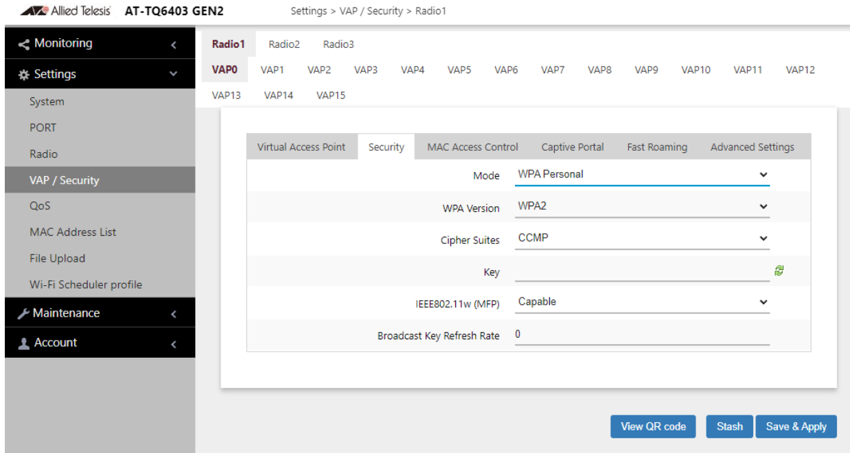
Figure 49. Security - WPA Personal
