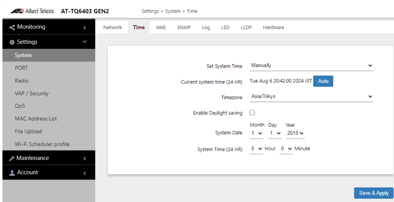
Figure 22. Time Window - Manual Option
