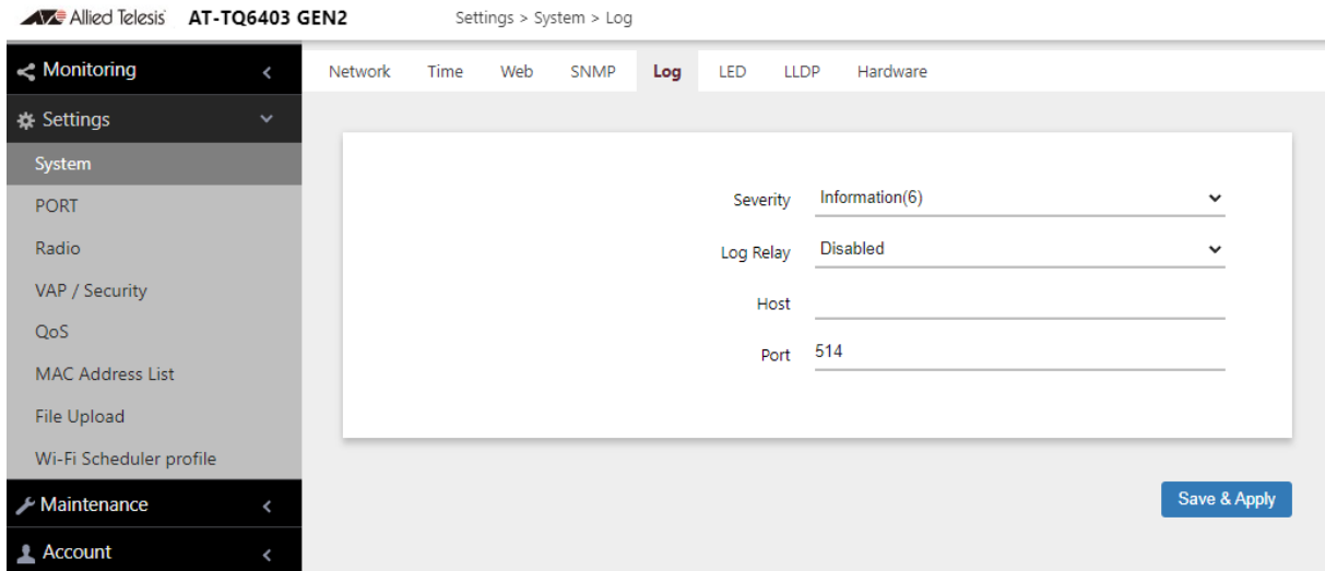
Figure 26. Log Window for Syslog Client
