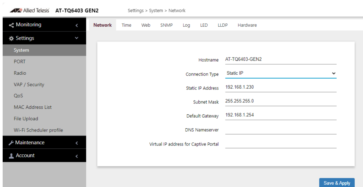
Figure 19. Network Static IP Address Window
