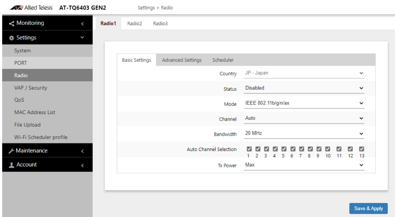
Figure 36. Basic Radio Settings Window
