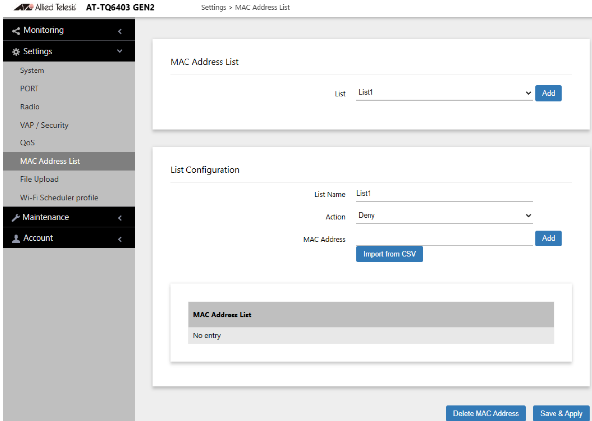
Figure 71. MAC Address List Window
