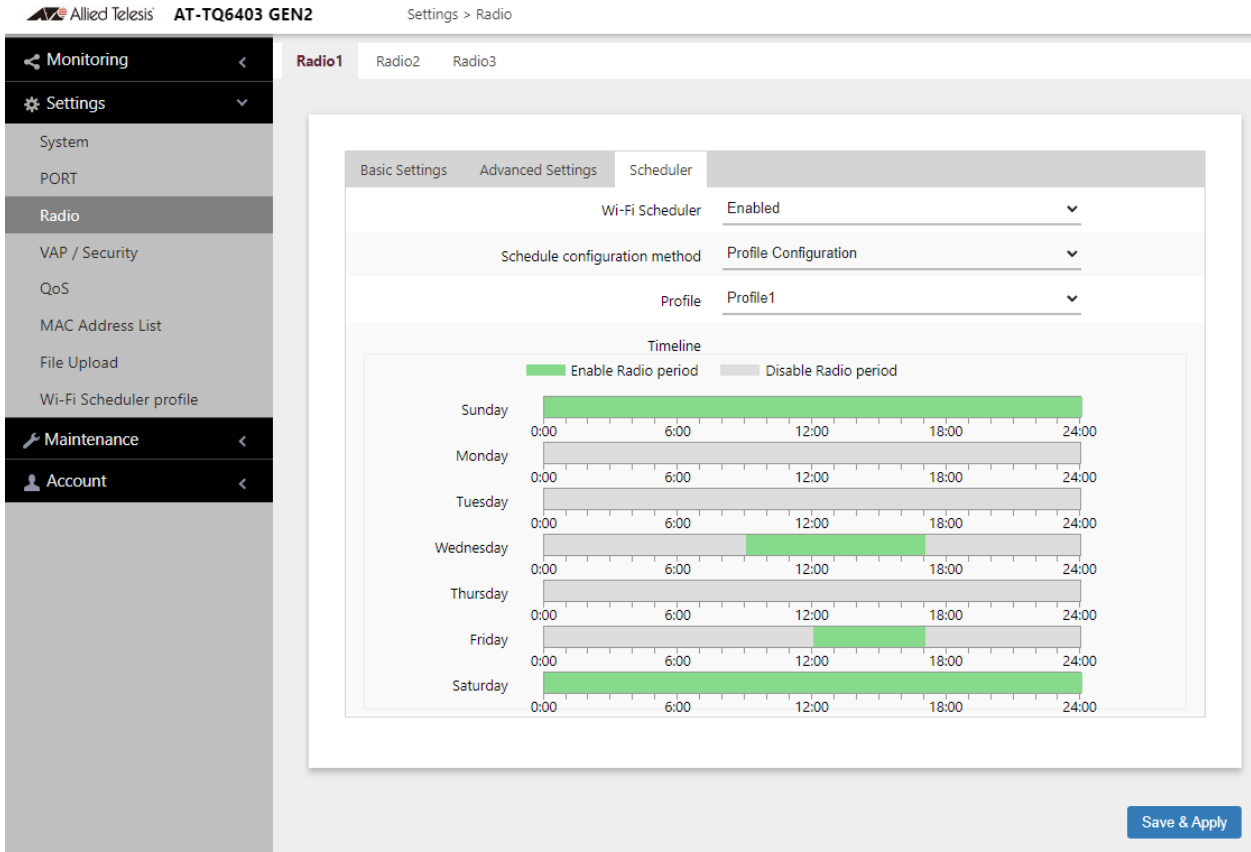
Figure 39. Assigning a Wi-Fi Scheduler Profile to a Radio
