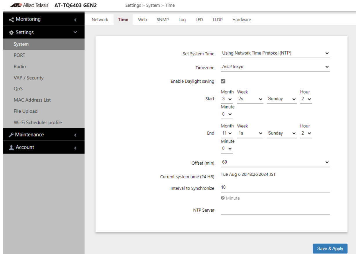
Figure 20. Time Window - NTP Option
