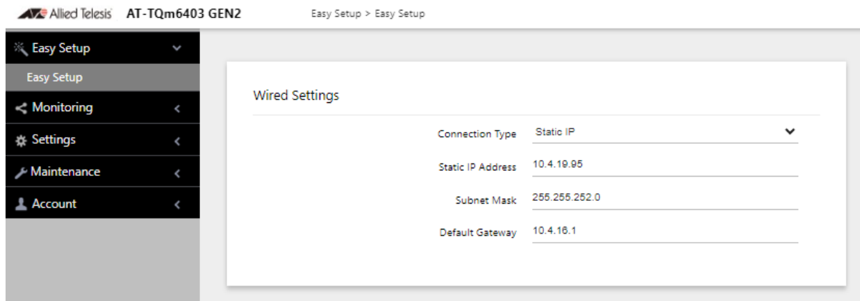
Figure 8. Easy Setup Page - Wired Settings - Static IP
