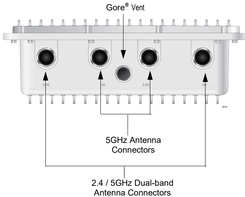
Figure 2. Rear Panel of the TQ6702e GEN2 Access Point
