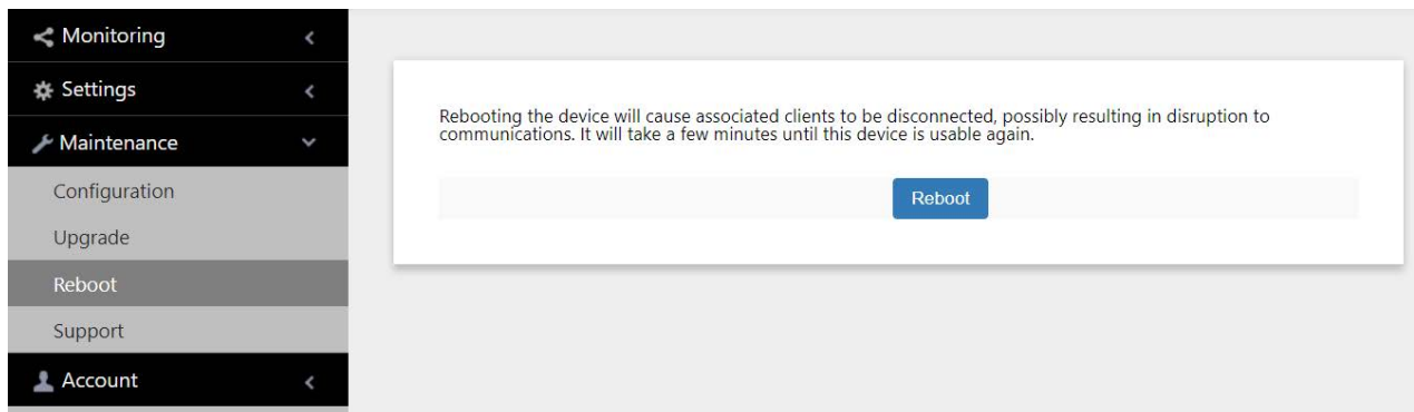
Figure 76. Reboot Window
