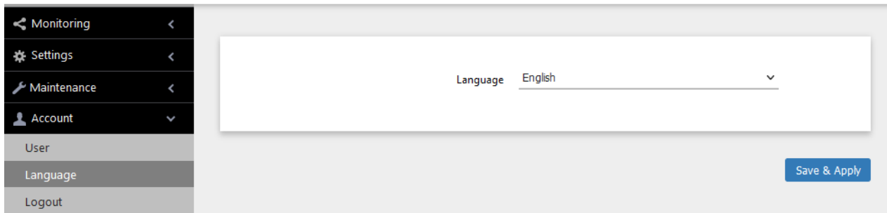
Figure 79. Language Window
