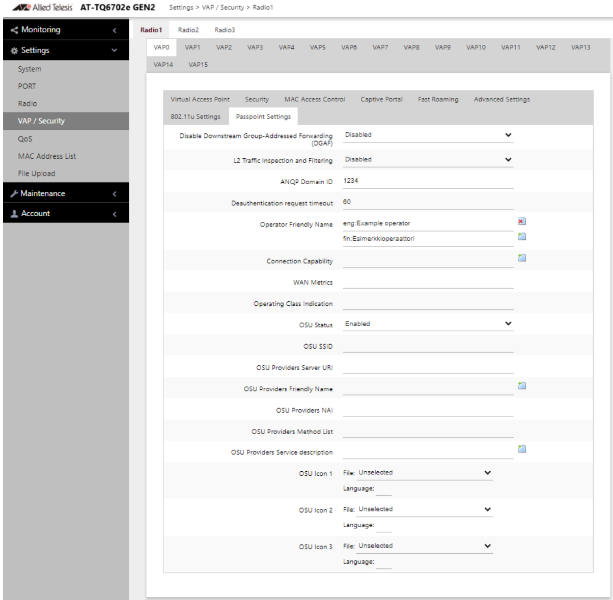
Figure 70. Passpoint Settings
