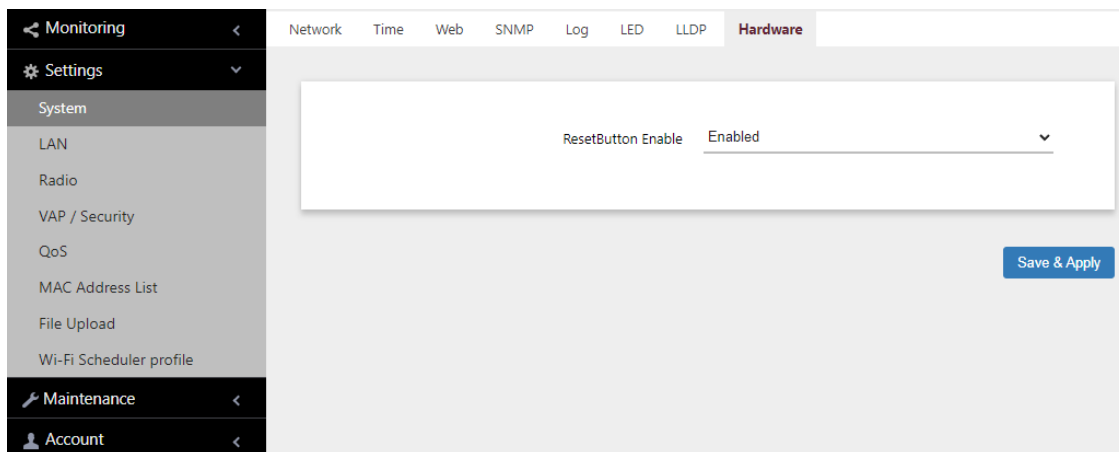
Figure 26. Hardware Window
