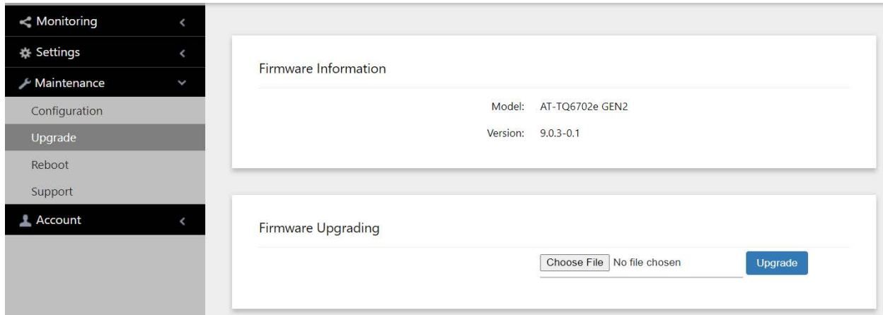
Figure 75. Upgrade Window
