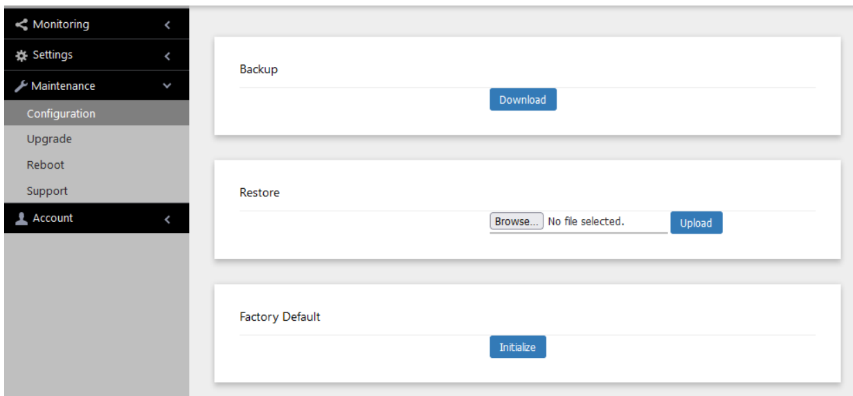
Figure 74. Configuration Window
