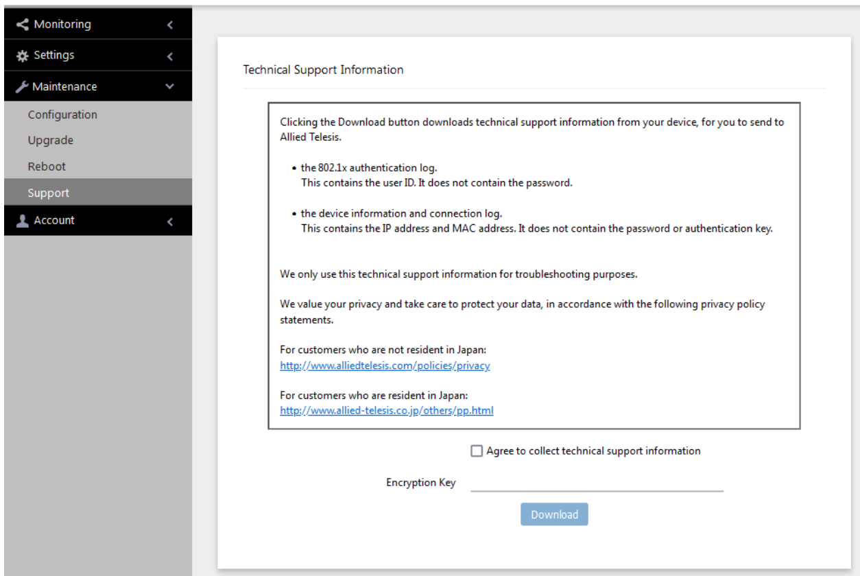
Figure 77. Support Window
