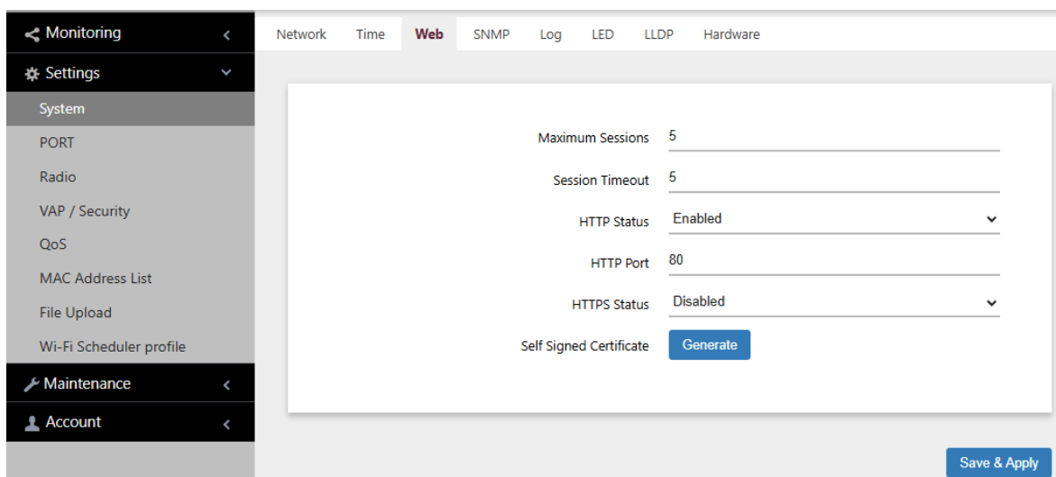
Figure 19. Web Window
