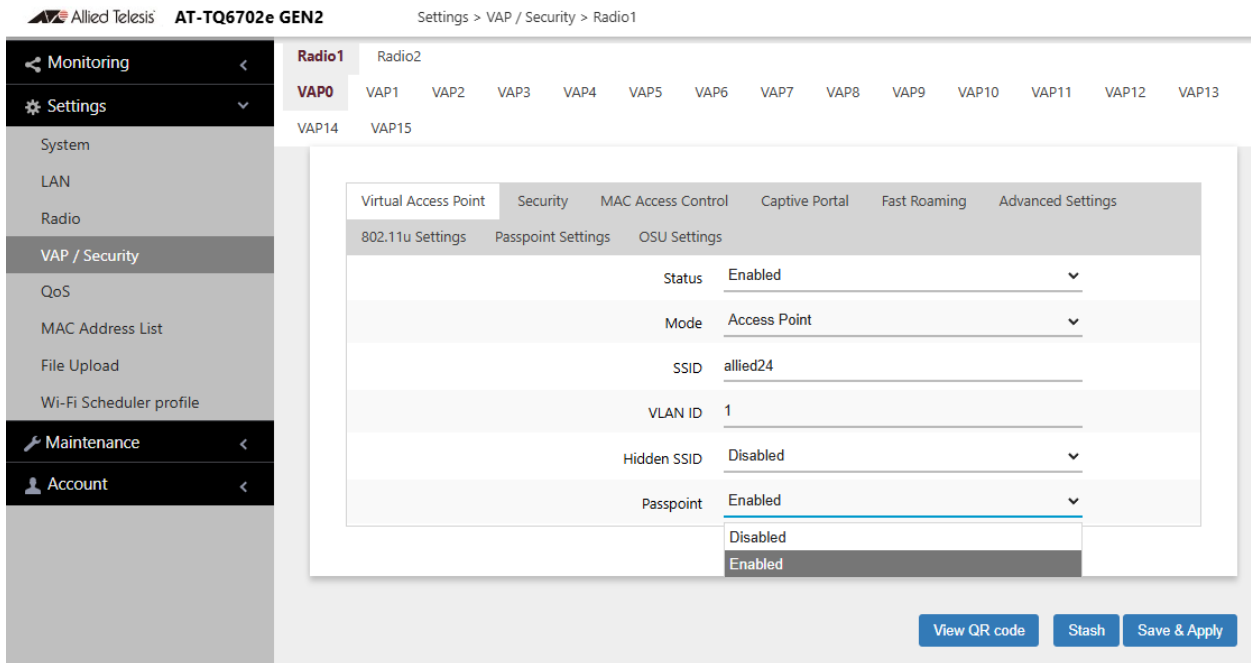
Figure 67. Enable/Disable Passpoint
