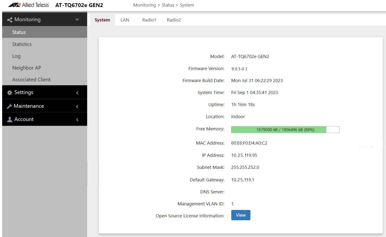
Figure 9. System Window
