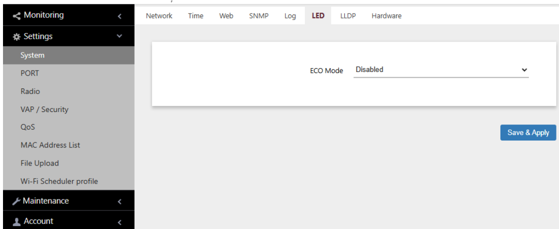
Figure 24. LED Window
