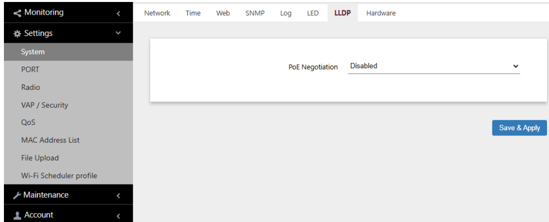
Figure 25. LLDP Window
