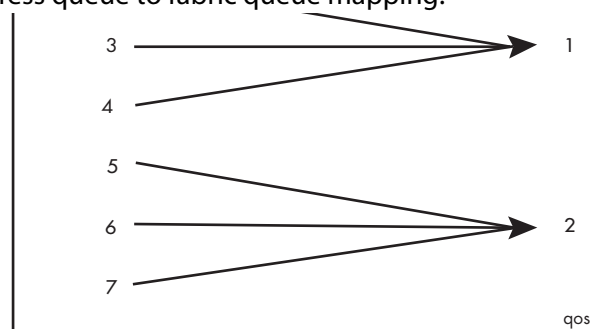
Figure 35-1: Egress queue to fabric queue mapping:
