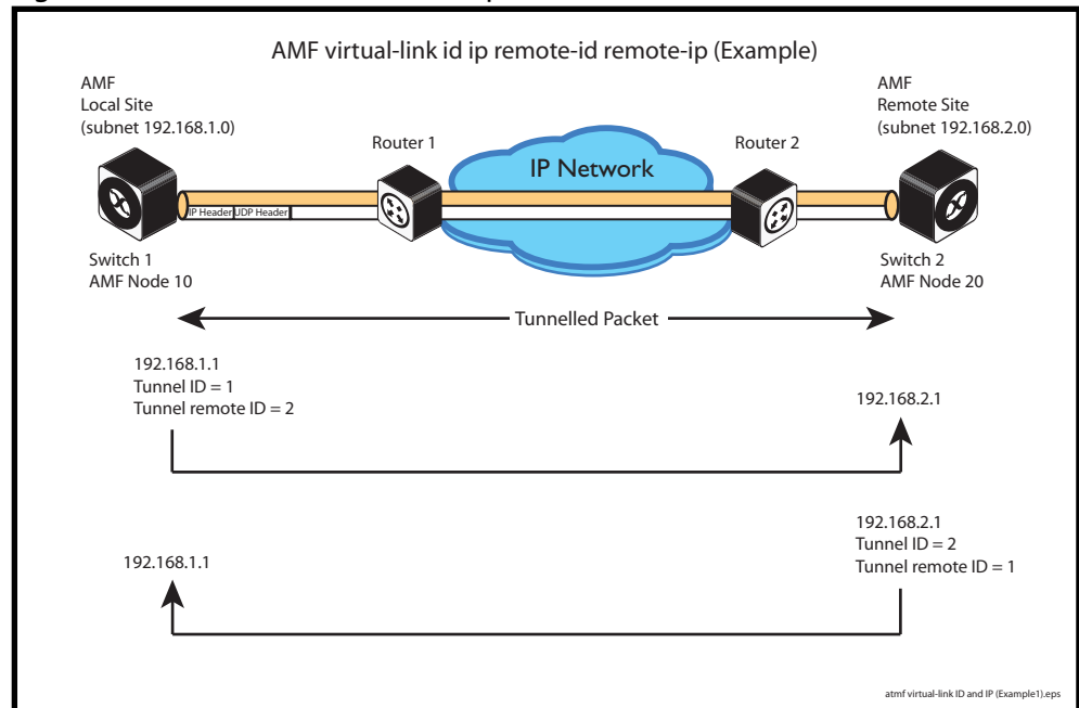
Figure 46-7: AMF virtual link example
